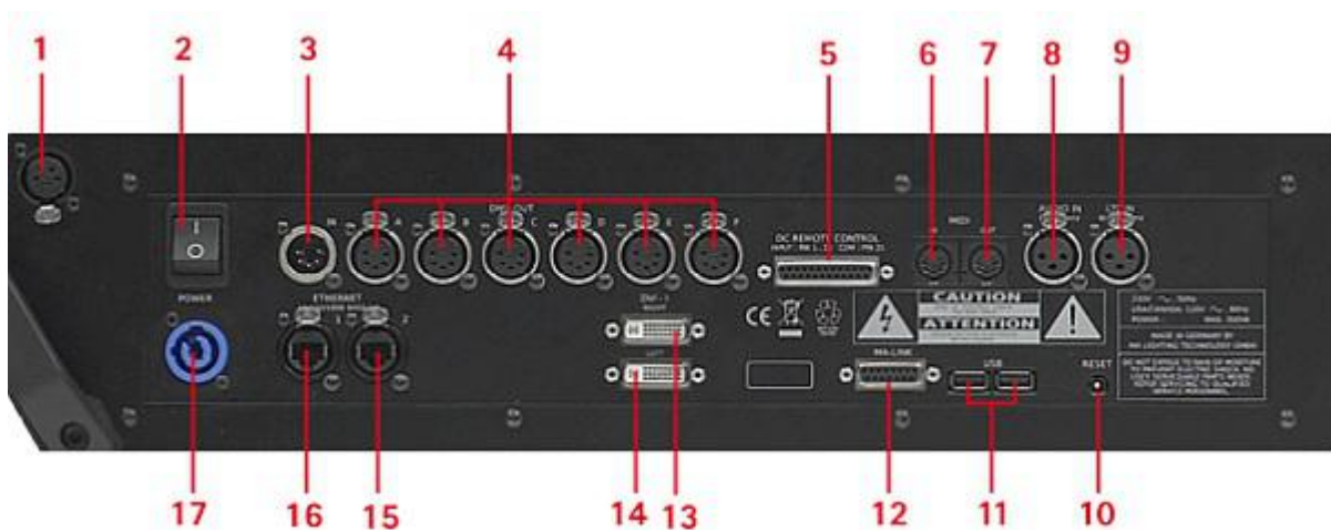
grandMA2 full-size rear panel in detail
