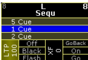
Two wide executor
